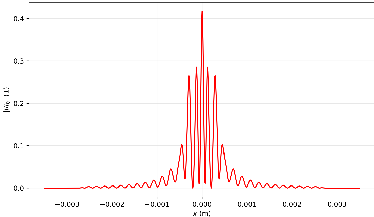
Intensity profile I(x, y = 0, z = 0.159)/I_0 , \text{Pin}=8.0\text{Pcr} , artificial time
